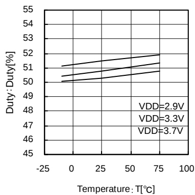
Fig.31 98MHz Temperature—Duty
