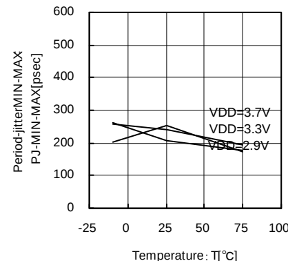
Fig.42 14.3MHz Temperature – Period-Jitter MIN-MAX
