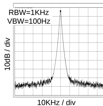
Fig.21 14.3MHz Spectrum At VDD=3.3V and CL=15pF
