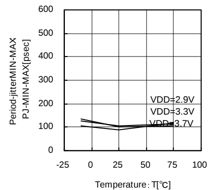
Fig.33 98MHz Temperature—Period-Jitter MIN-MAX
