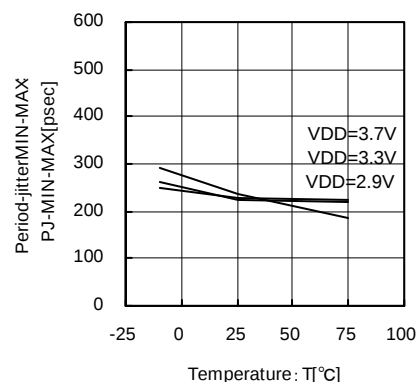
Fig.39 17.7MHz Temperature – Period-Jitter MIN-MAX
