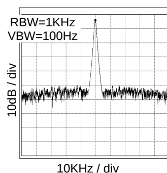
Fig.18 17.7MHz Spectrum At VDD=3.3V and CL=15pF
