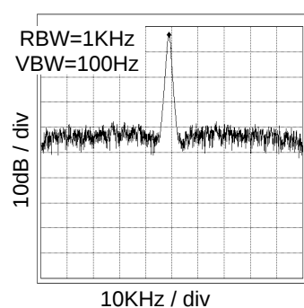
Fig.6 110MHz Spectrum At VDD=3.3V and CL=15pF
