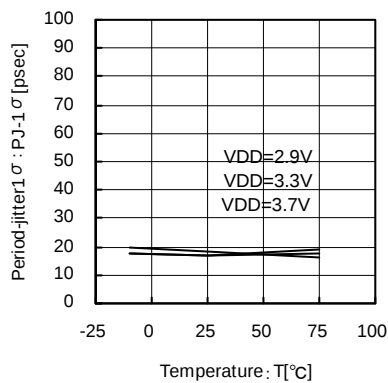
Fig.32 98MHz Temperature—Period-Jitter 1 \sigma
