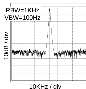
Fig.15 48MHz Spectrum At VDD=3.3V and CL=15pF
