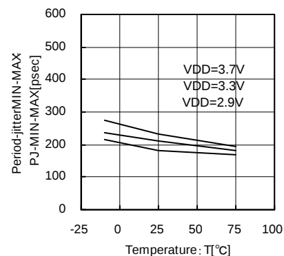
Fig.36 98MHz Temperature – Period-Jitter MIN-MAX
