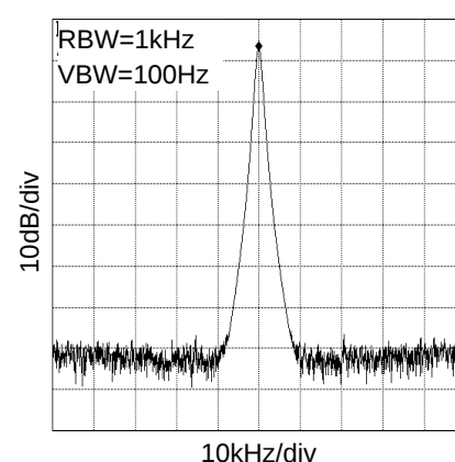
Fig.5 48.000MHz Spectrum VDD_CLK=2.6V, at CL=15pF
