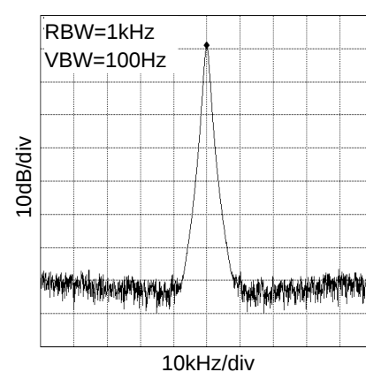
Fig.8 24.576MHz Spectrum VDD_CLK=1.8V, at CL=15pF
