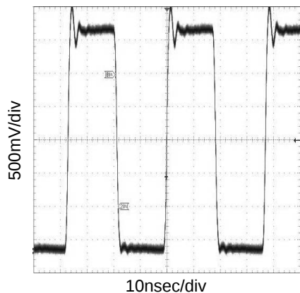
Fig.9 27.000MHz output waveform VDD_CLK=3.3V, at CL=15pF
