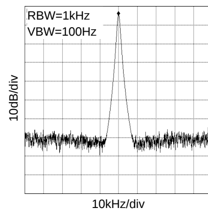
Fig.11 27.000MHz Spectrum VDD_CLK=3.3V, at CL=15pF
