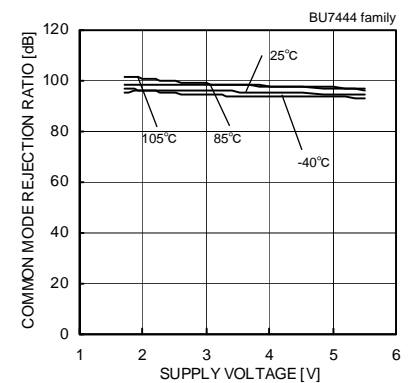
Fig.156 Common Mode Rejection Ratio – Supply Voltage
