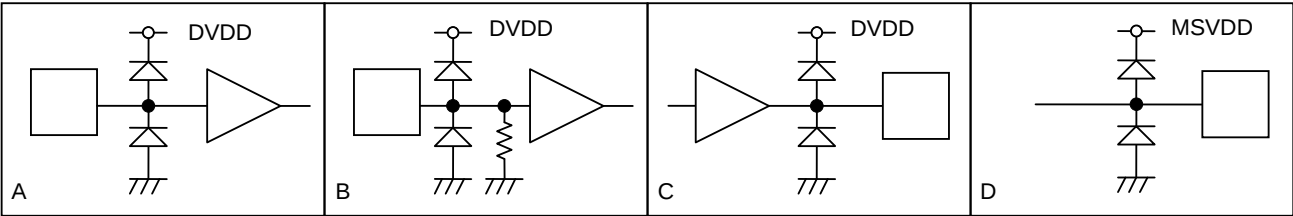
Fig.4. Equivalent Schematics
