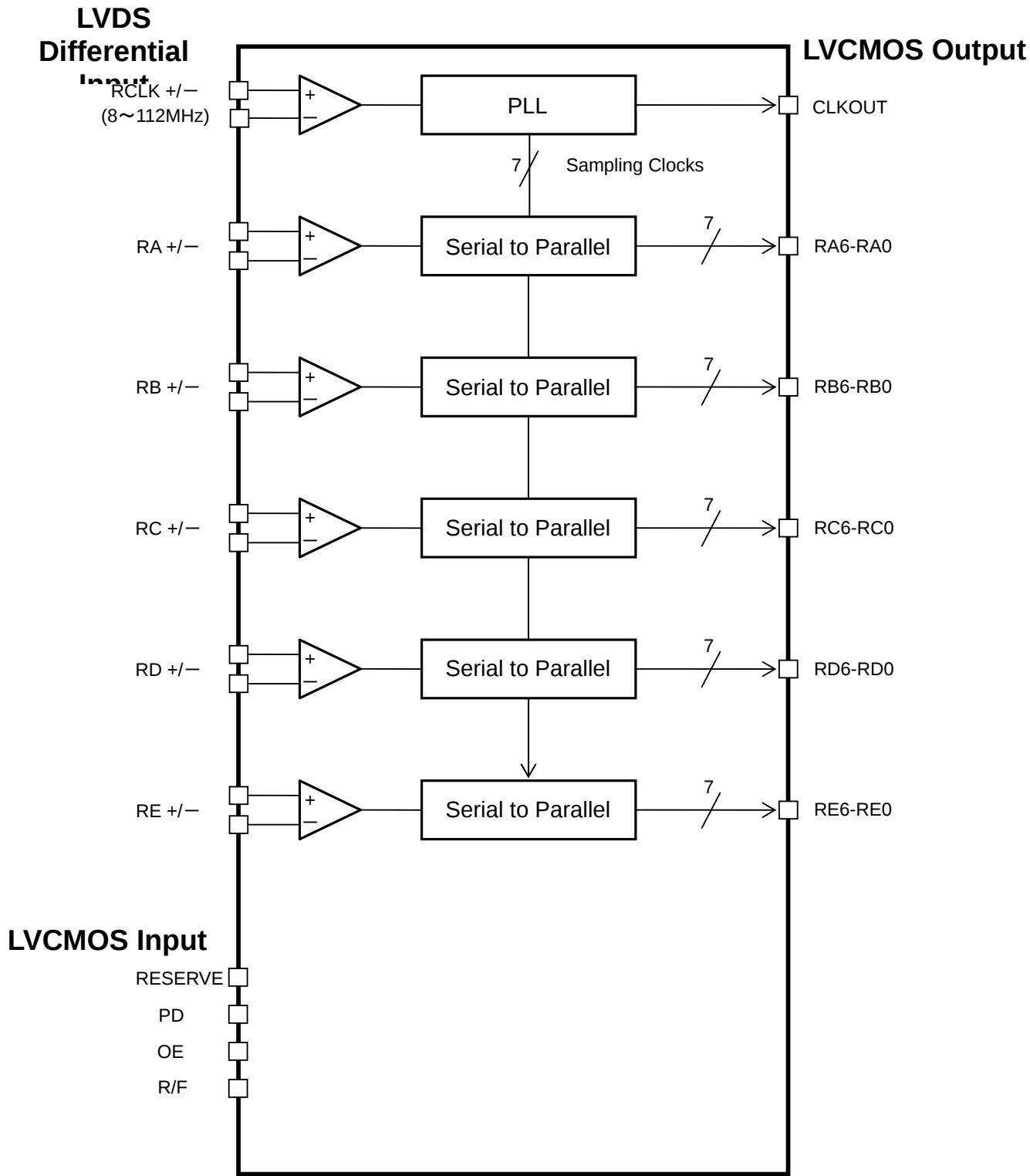
Fig.1 Block Diagram
