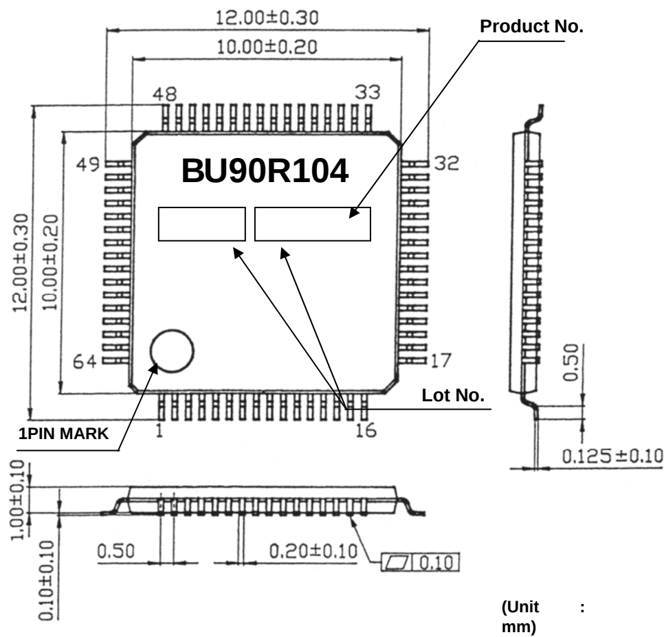
Fig.2 TQFP64V Package
