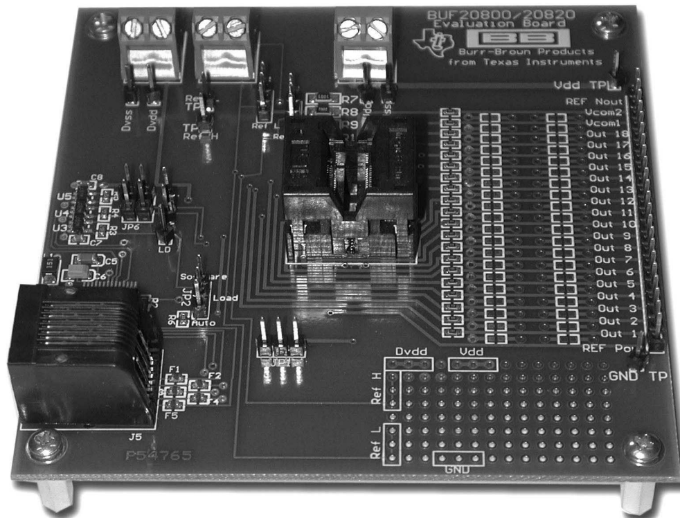
Figure 19. Evaluation Board
