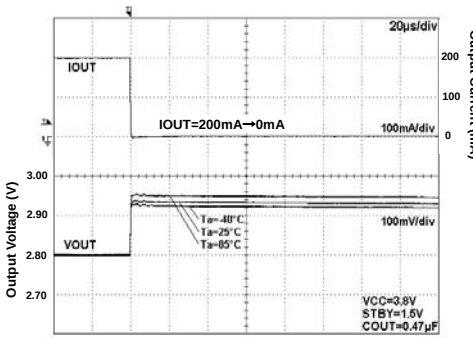
Fig 198. Load Response
