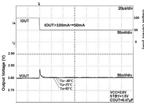
Fig 200. Load Response
