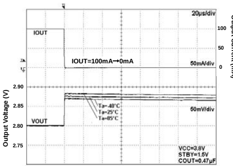
Fig 196. Load Response
