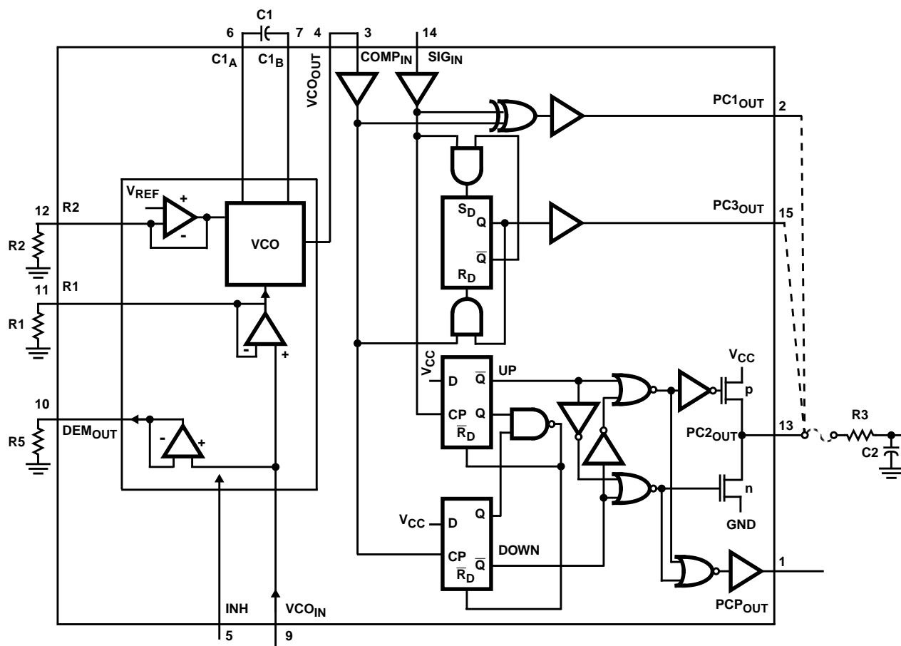
FIGURE 1. LOGIC DIAGRAM
