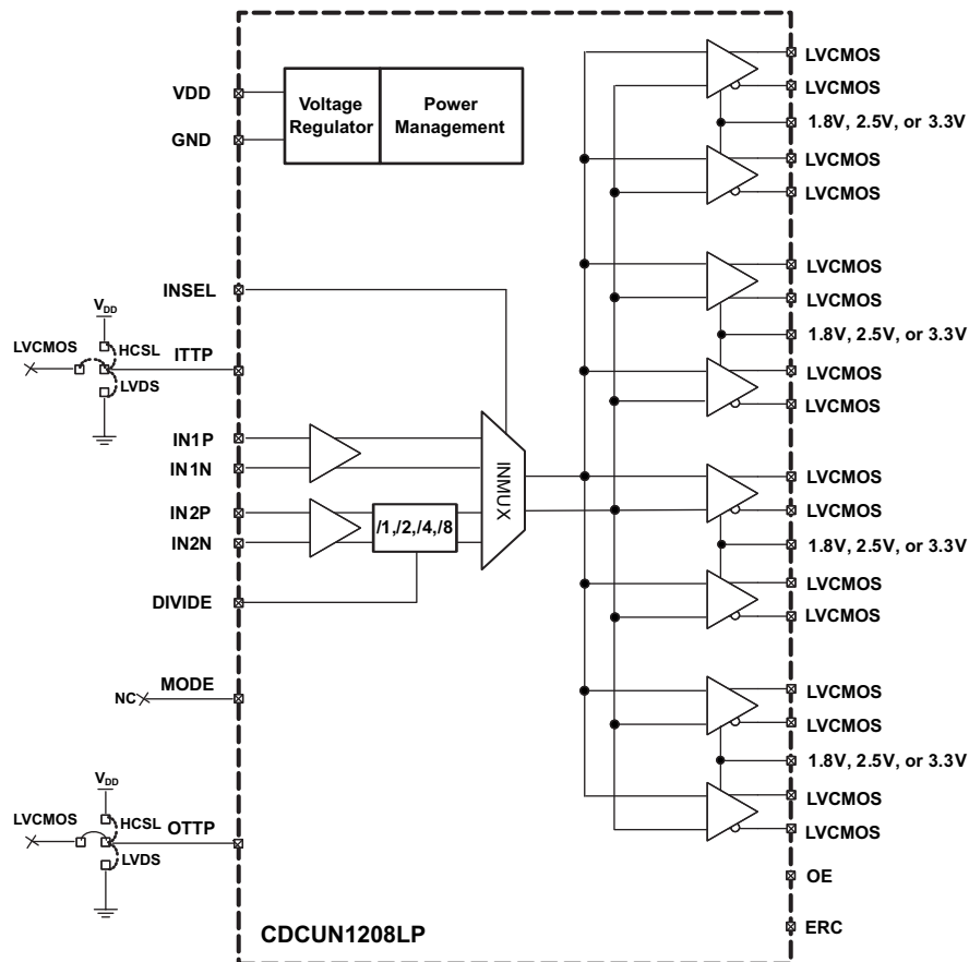
Figure 2. CDCUN1208LP Typical Application Example – LVC MOS Output Mode
