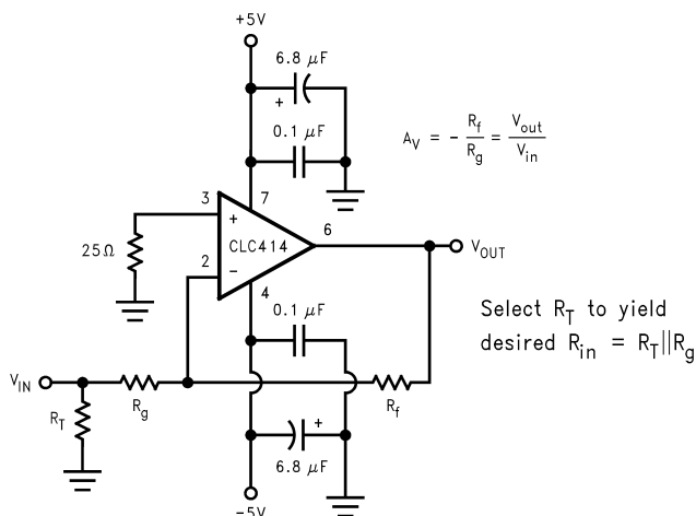
Figure 20. Recommended Inverting Gain Circuit
