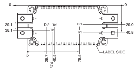
T1 / T2: IGBT, D1 / D2: FWDi, Th: NTC Thermistor Each mark points to the center position of each chip.
