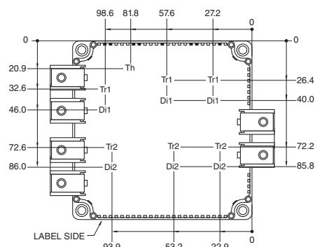
Tr1 / Tr2: IGBT, Di1 / Di2: FWDi, Th: NTC Thermistor Each mark points to the center position of each chip.
