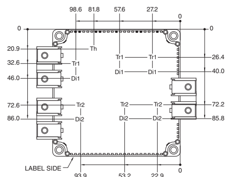
Tr1 / Tr2: IGBT, D1 / D2: FWDI, Th: NTC Thermistor Each mark points to the center position of each chip.
