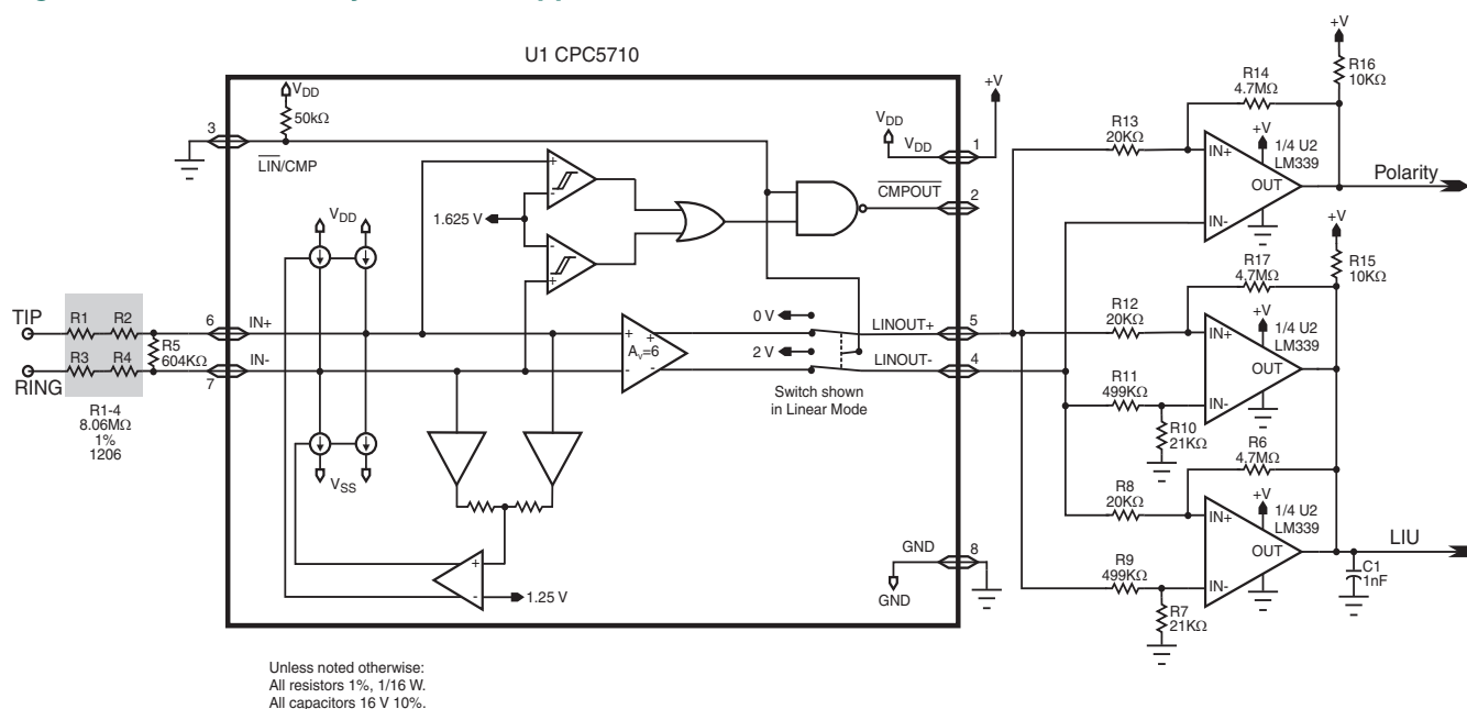
Figure 4. LIU and Polarity Detection Application Circuit
