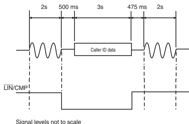
Figure 1. LIN/CMP Timing for Caller-ID Signal Reception
