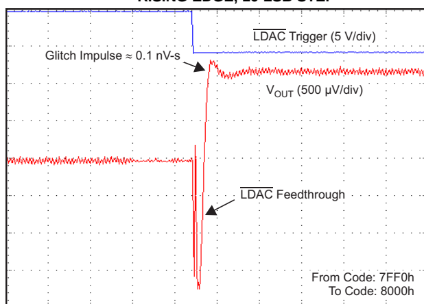
GLITCH ENERGY RISING EDGE, 16-LSB STEP
