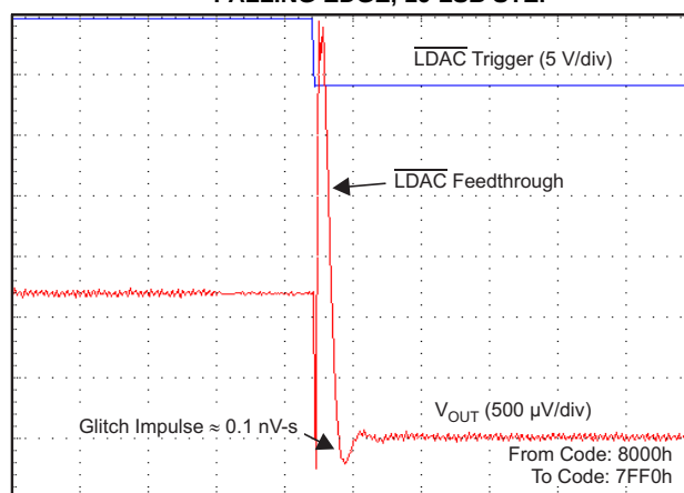
GLITCH ENERGY FALLING EDGE, 16-LSB STEP
