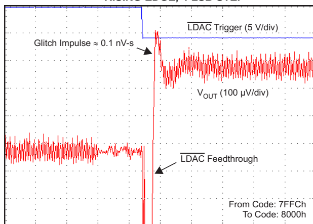
GLITCH ENERGY RISING EDGE, 4-LSB STEP
