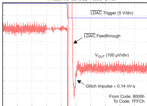
GLITCH ENERGY FALLING EDGE, 4-LSB STEP
