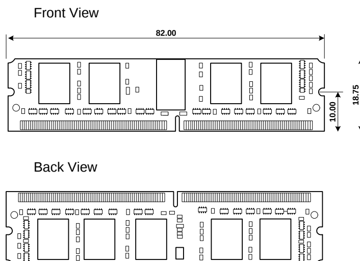
Figure: mechanical dimensions 1
