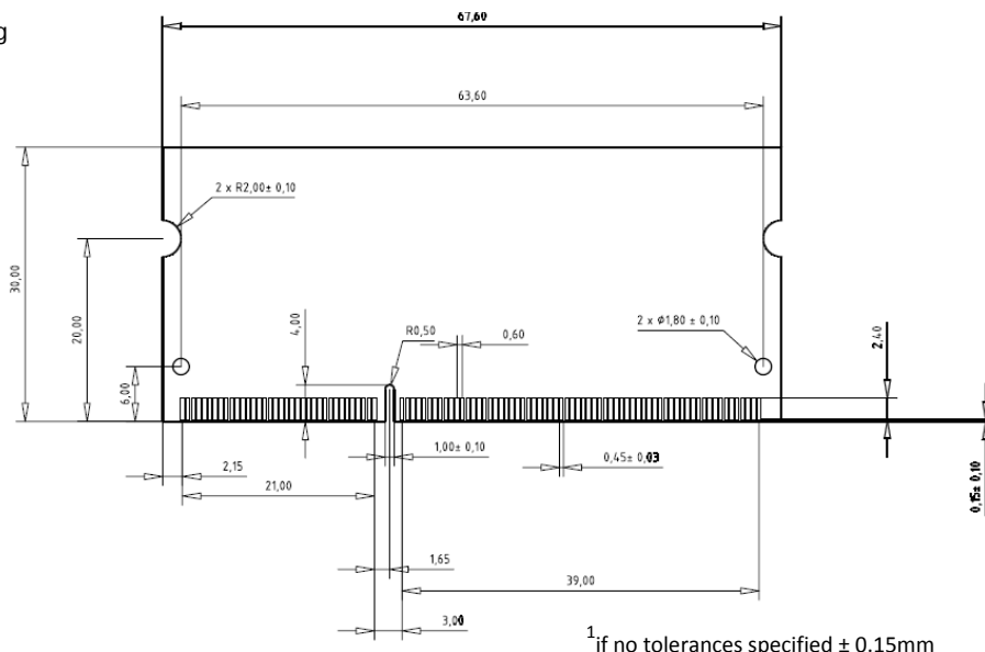
Figure: mechanical dimensions 1
