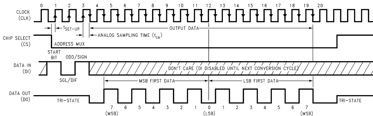
Figure 17. ADC08034 Timing
