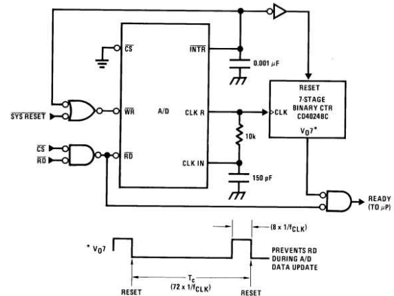
Figure 23. µP Interface for Free-Running A/D
