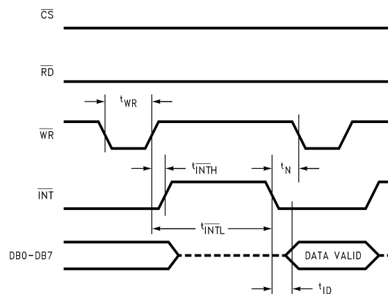
Figure 4. \overline{\text{WR}}\text{-}\overline{\text{RD}} Mode Reduced Interface System Connection with \overline{\text{CS}} = \overline{\text{RD}} = 0 (Mode Pin is High)
