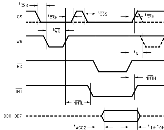
Figure 3. \overline{\text{WR}}\text{-}\overline{\text{RD}} Mode with t_{\text{RD}} > t_{\text{INTL}} (Mode Pin is High)
