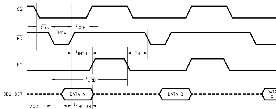
Figure 5. \overline{\text{RD}} Mode (Pipeline Operation); t_{\text{RDW}} must be between 200 ns and 400 ns. (Mode Pin is Low)
