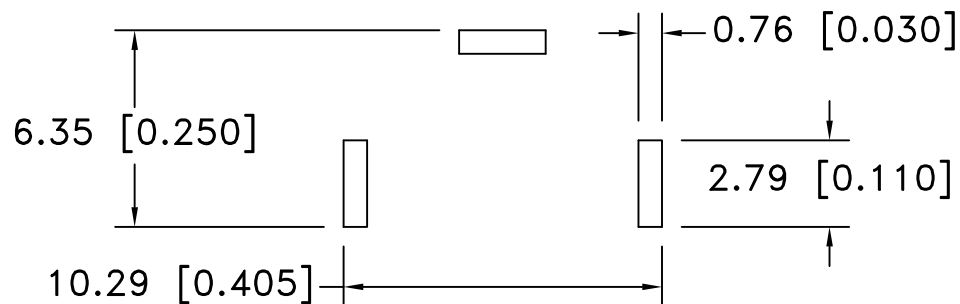
PCB LAYOUT
