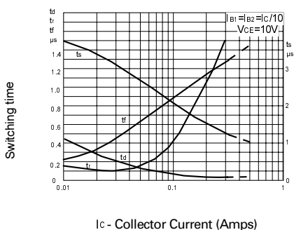
Switching Speeds
