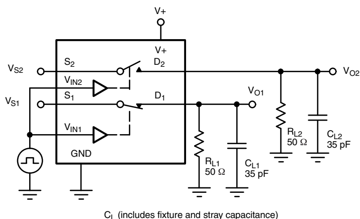
Figure 2. Break-Before-Make (DG2739)
