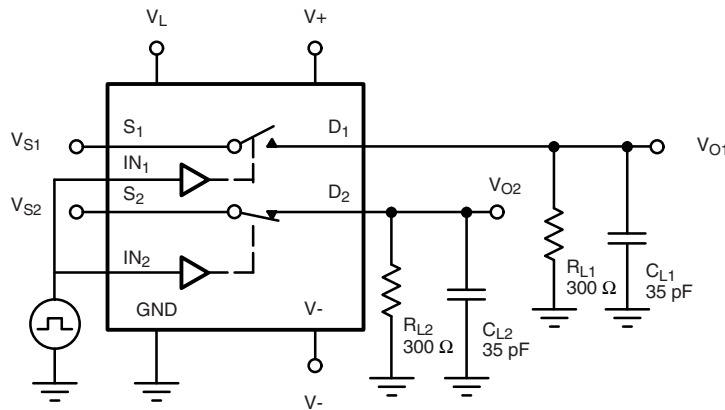
Figure 3. Break-Before-Make (DG413L)
