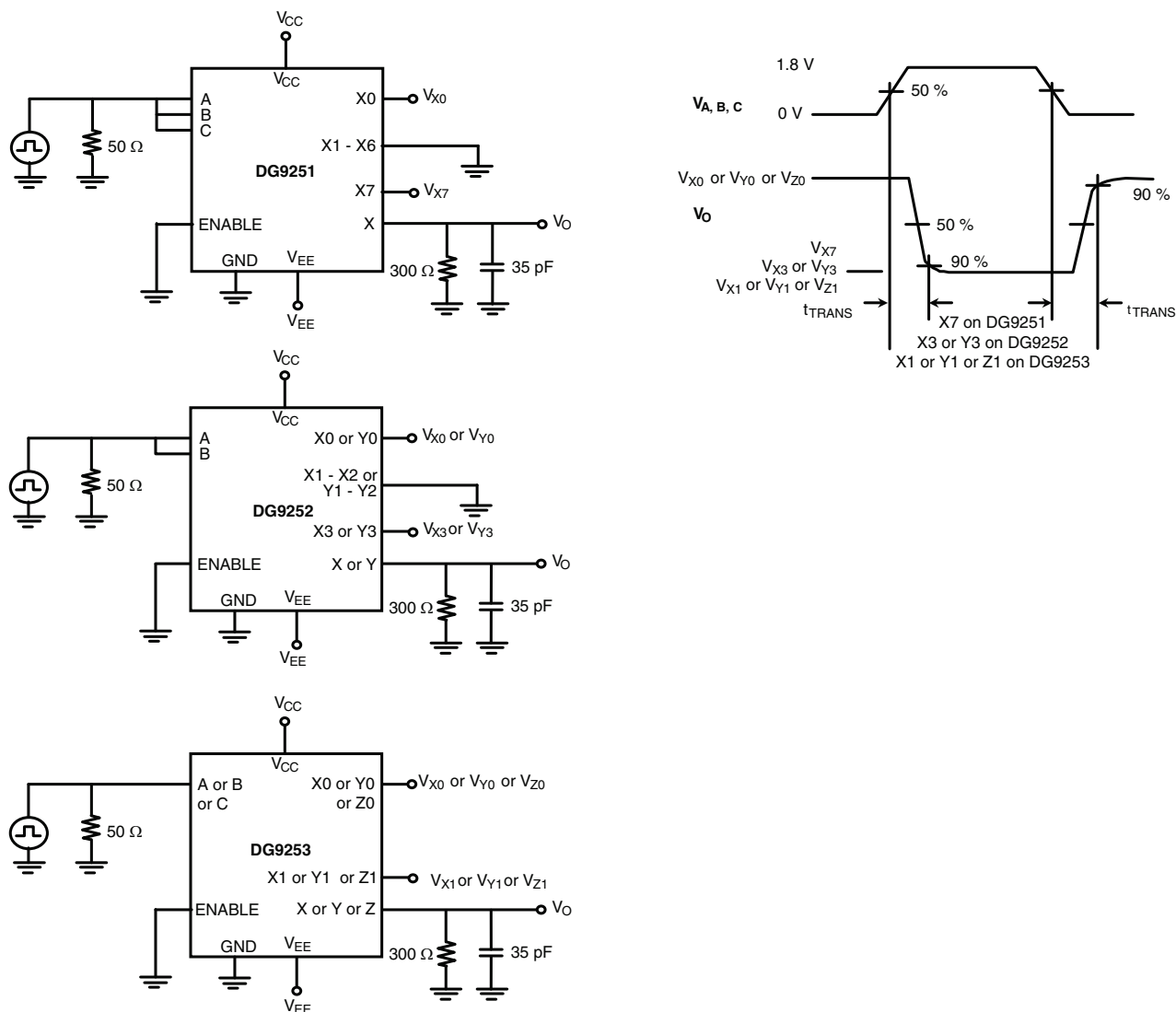
Figure 1. Transition Time
