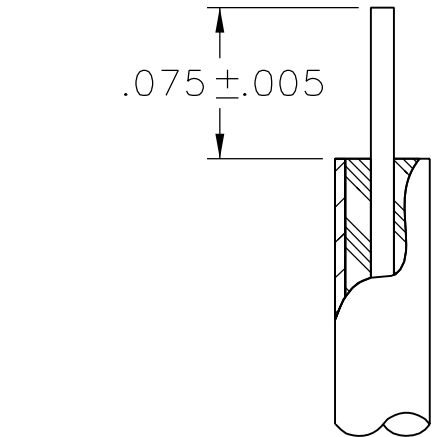
CABLE STRIP DIMENSIONS 10:1
