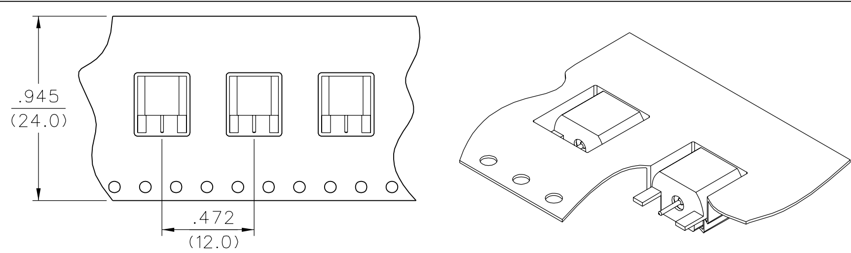
FIG 1 2:1 TOP VIEW
