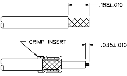
CABLE STRIP DIMENSIONS
