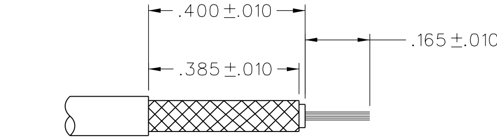
CABLE STRIP DIMENSIONS NOT TO SCALE
