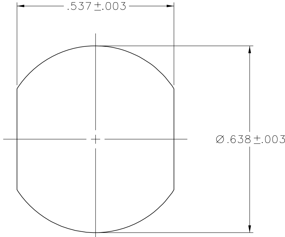
MOUNTING HOLE
