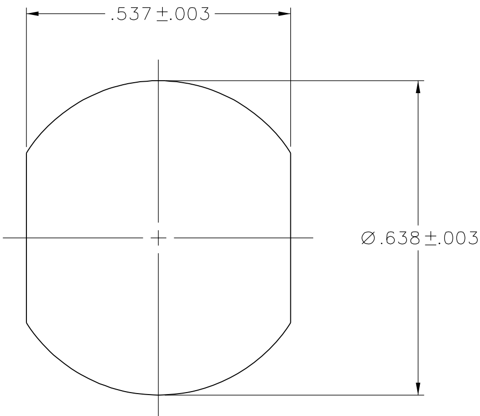
MOUNTING HOLE
