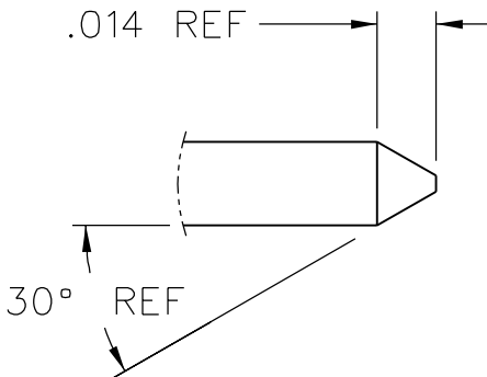
POINTING DETAIL 20:1
