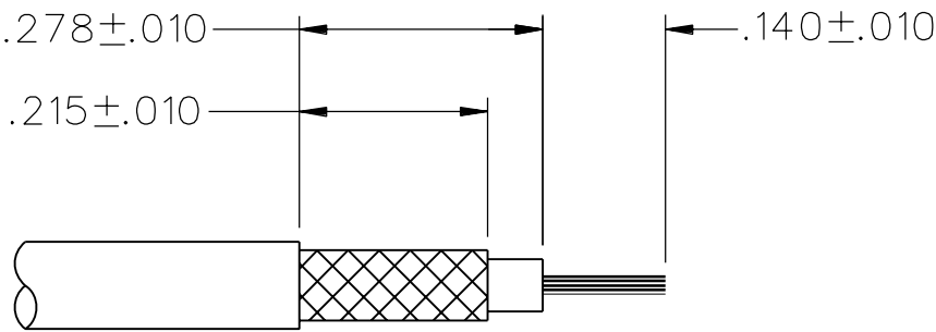
CABLE STRIP DIMENSIONS 4:1
