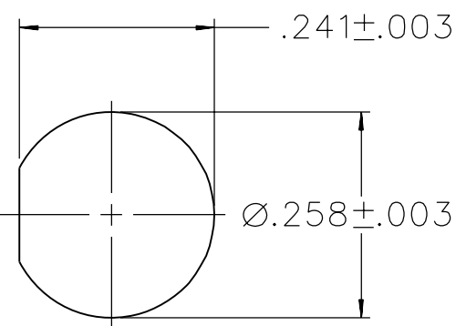
MOUNTING HOLE 4:1
