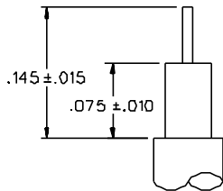
CABLE STRIP DIMENSIONS
