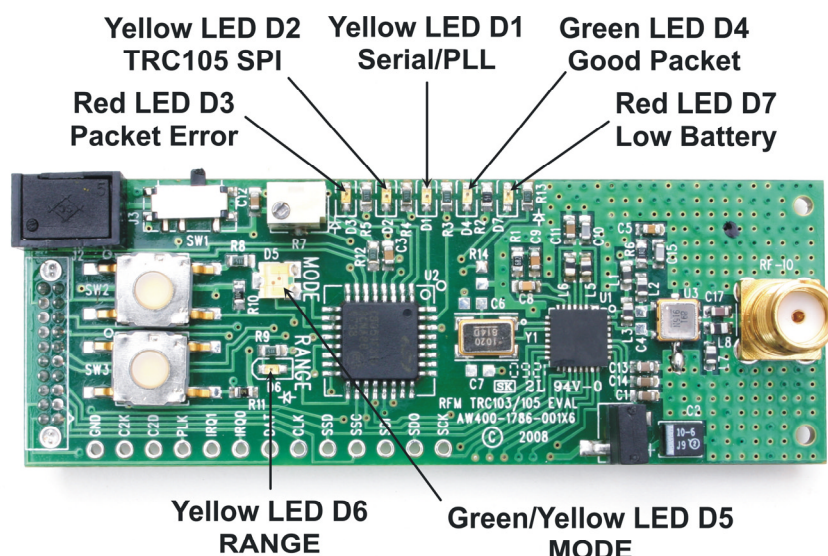
Figure 2 - DR-TRC105 Radio Board LED Indicators
