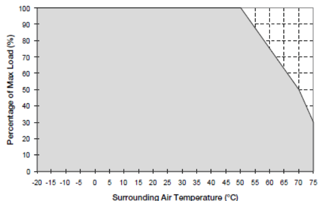
Fig. 1.2 De-rating for Vertical Mounting Orientation > 50°C de-rate power by 2.5% / °C, > 70°C de-rate power by 4% / °C
