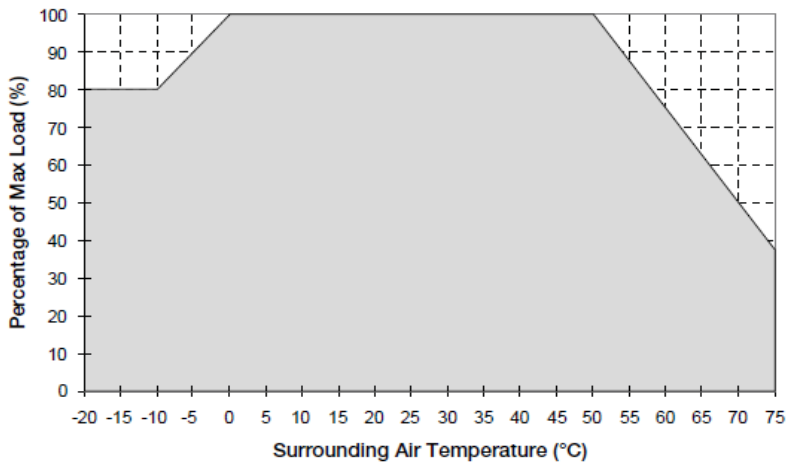
Fig. 1.1 De-rating for Vertical Mounting Orientation < 0°C to -20°C de-rate power by 1% / °C, > 50°C de-rate power by 2.5% / °C
