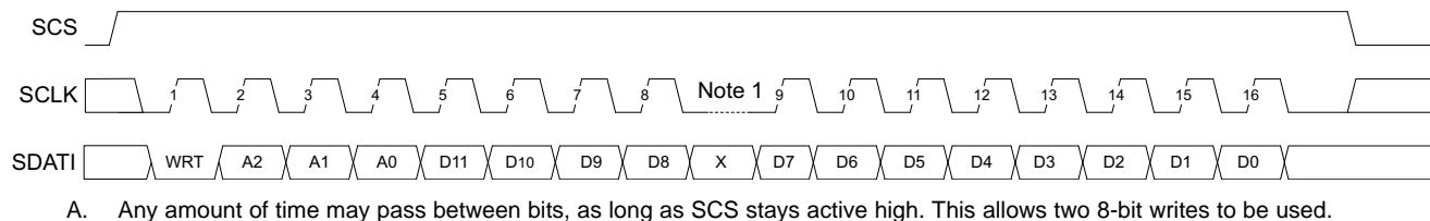
Figure 10. Write Operation
