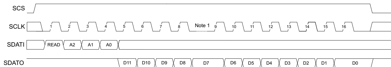
Figure 11. Read Operation
