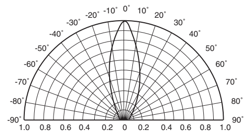
Fig. 4 Radiation Diagram
