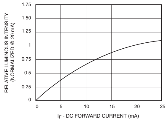
Fig.2 Relative Luminous Intensity vs. DC Forward Current
