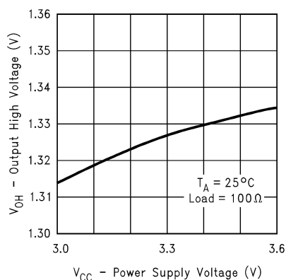
Figure 9. Output High Voltage vs Power Supply Voltage
