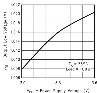
Figure 10. Output Low Voltage vs Power Supply Voltage
