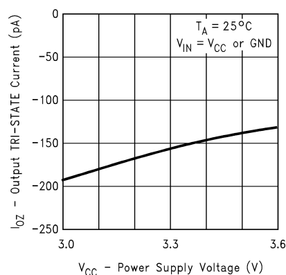
Figure 12. Output TRI-STATE Current vs Power Supply Voltage
