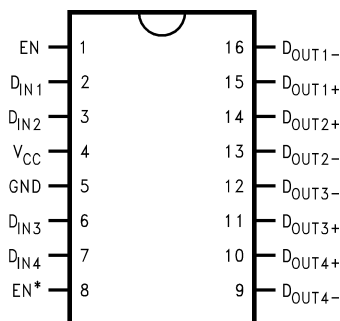
Figure 1. Order Number DS90LV047ATM, DS90LV047ATMTC D0016A, PW0016A Packages
