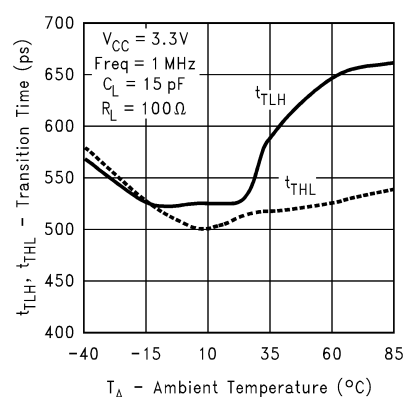
Figure 24. Transition Time vs Ambient Temperature
