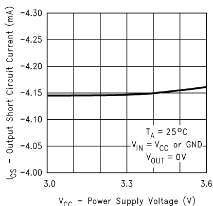
Figure 11. Output Short Circuit Current vs Power Supply Voltage
