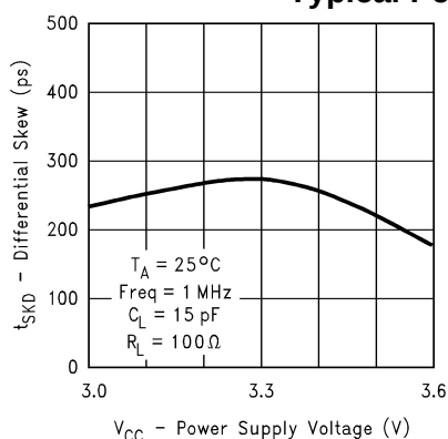
Figure 21. Differential Skew vs Power Supply Voltage
