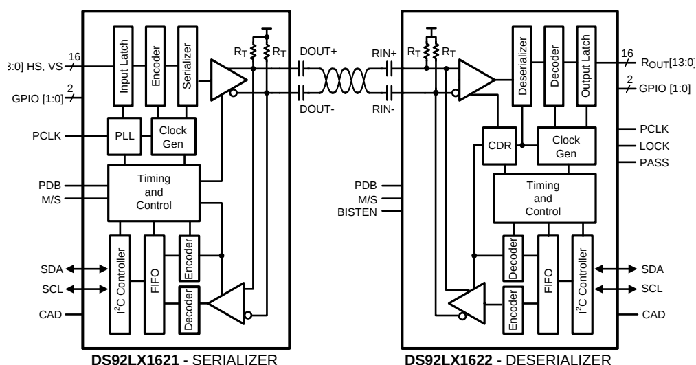
Figure 2. Block Diagram
