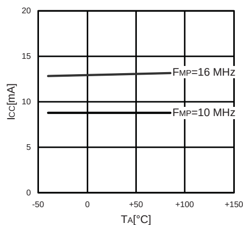
I_{CCS} - T_A V_{CC} = 5.5 V, F_{MP} = 10, 16 MHz (divided by 2) Main sleep mode with the external clock operating
