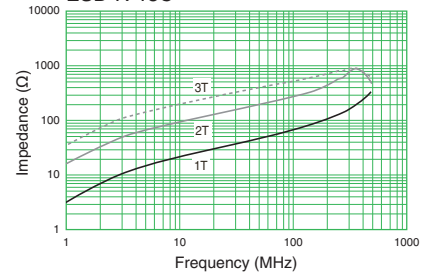
ESD-R-19E-1
