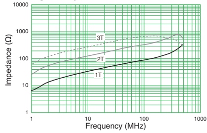
ESD-R-10S
