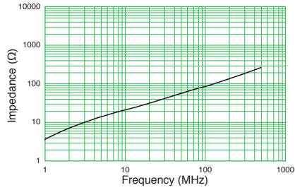
ESD-FPD-40,40-1
