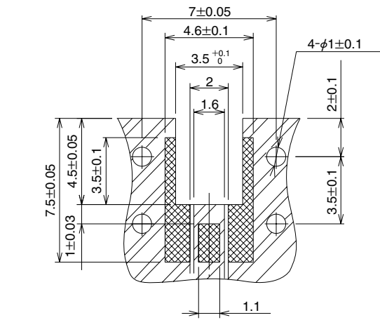
PCB mounting pattern (MMCX-LR-SMT) (Reference) Glass epoxy FR-4 t=0.8 (■=4.6)
