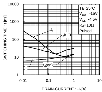
Fig.11 Switching Characteristics
