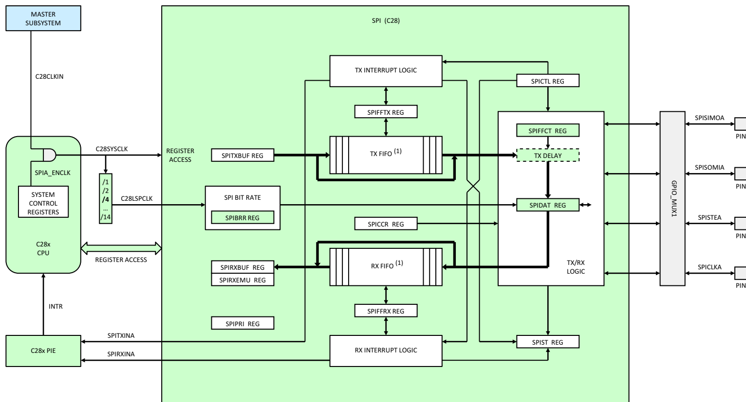
Figure 6-41. SPI (C28x)
