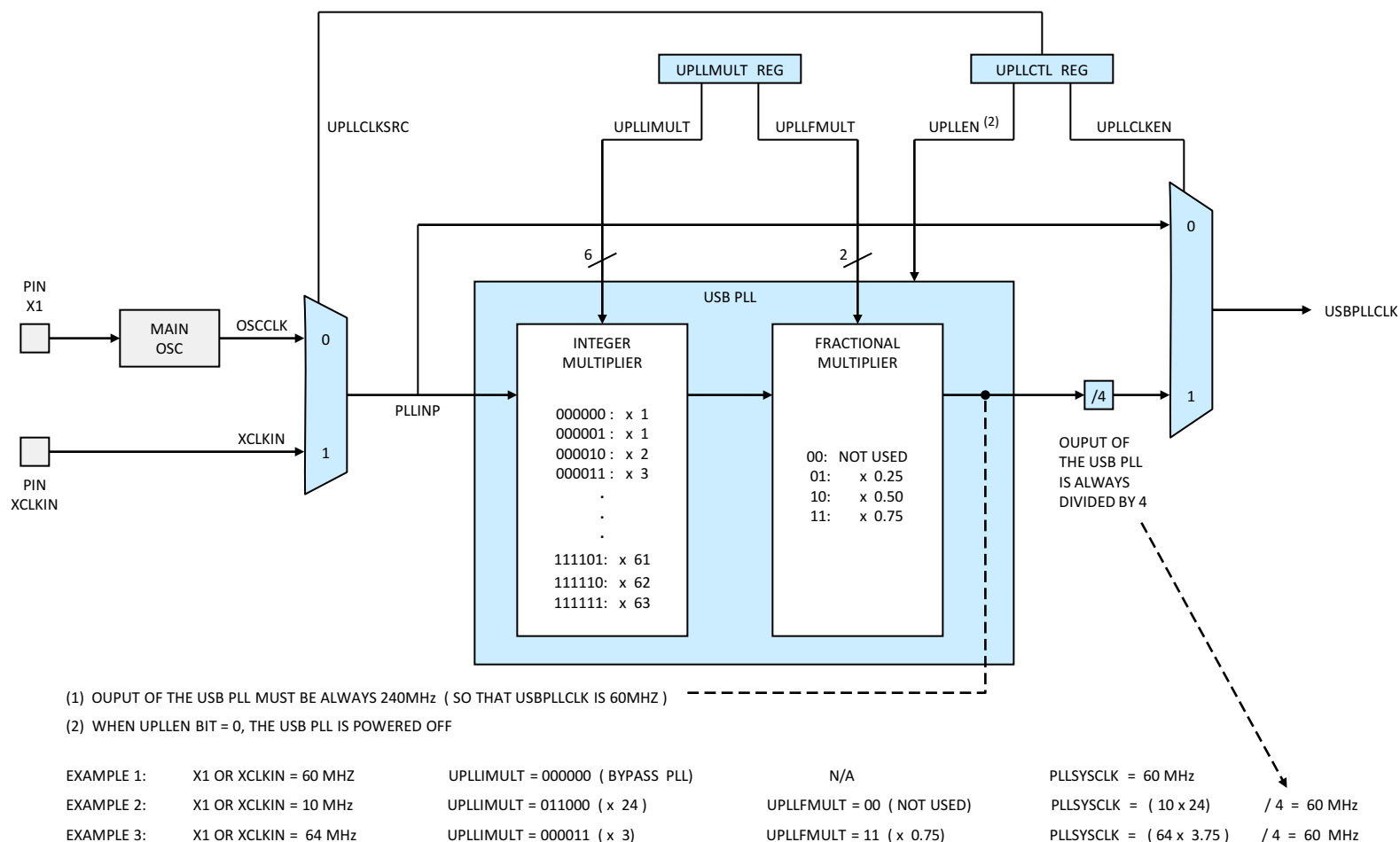
Figure 2-9. USB PLL
