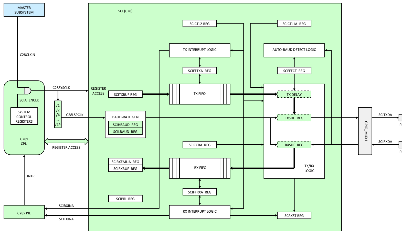
Figure 6-40. SCI (C28x)
