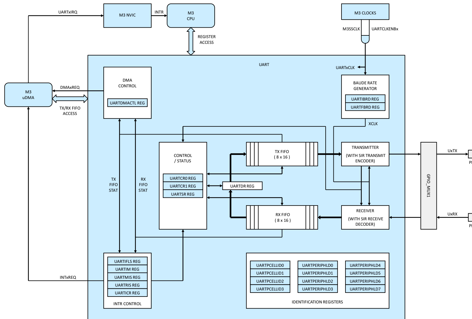
Figure 6-22. UART
