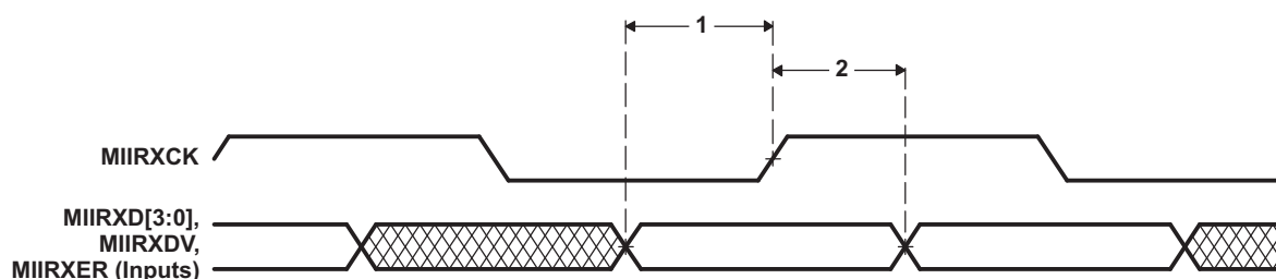
Figure 6-30. 100/10Mb/s MII Receive Timing
