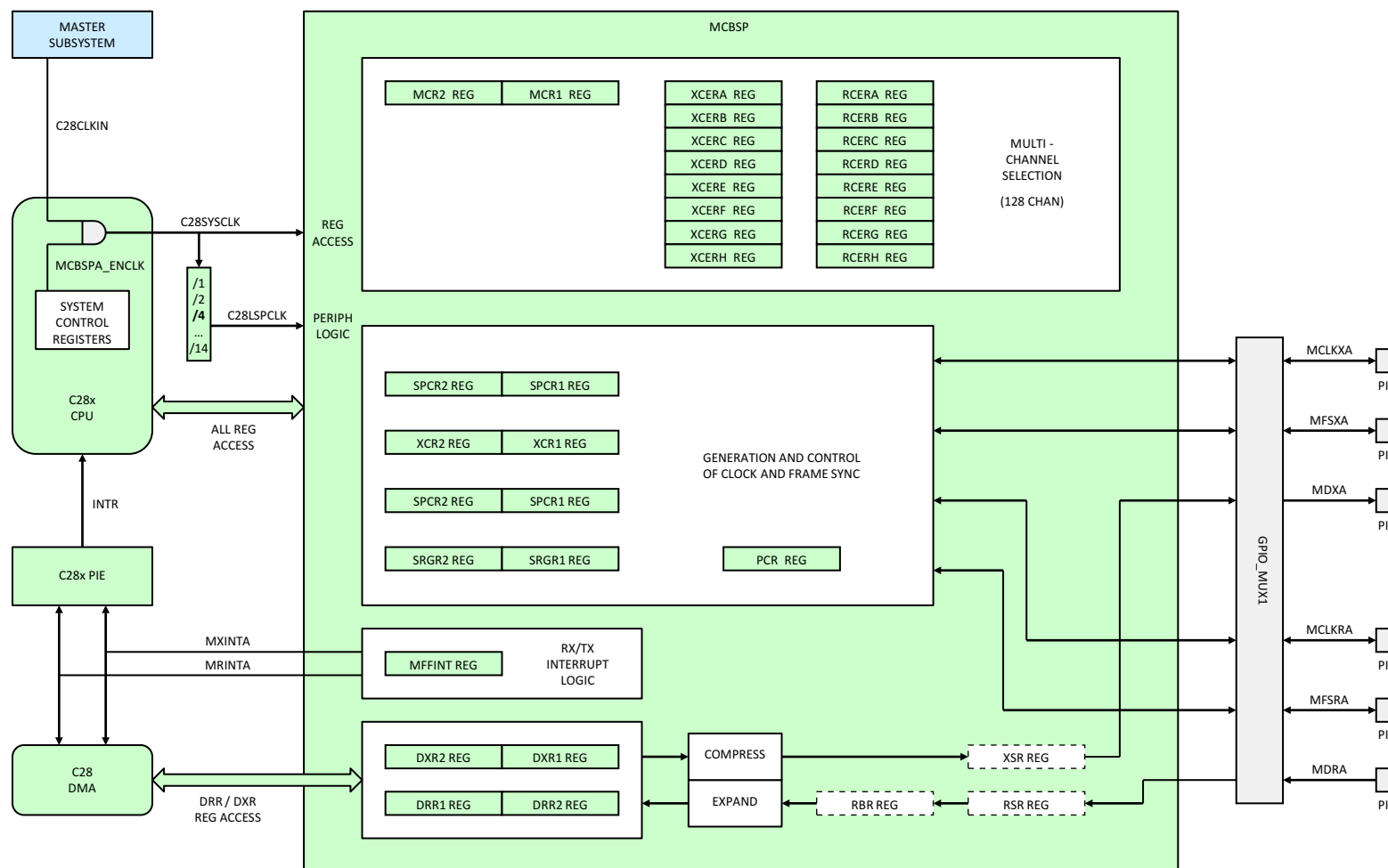
Figure 6-46. McBSP (C28x)
