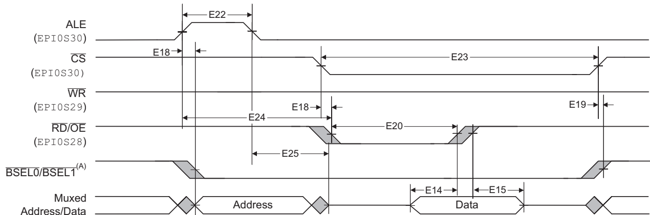
Figure 6-17. Host-Bus 8/16 Mode Muxed Read Timing
