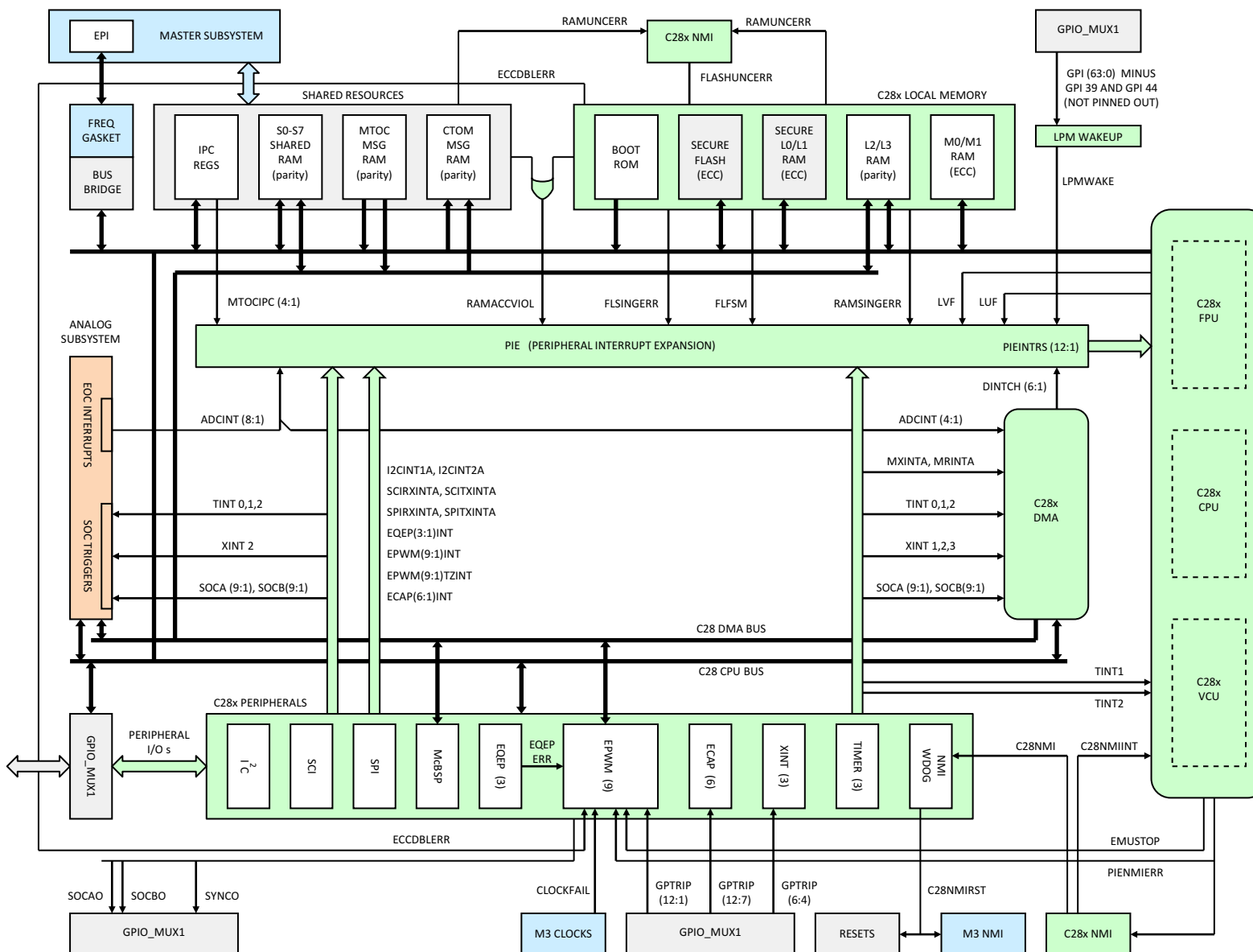
Figure 2-2. Control Subsystem
