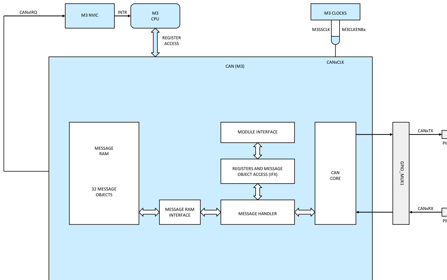
Figure 6-24. CAN (Cortex™-M3)
