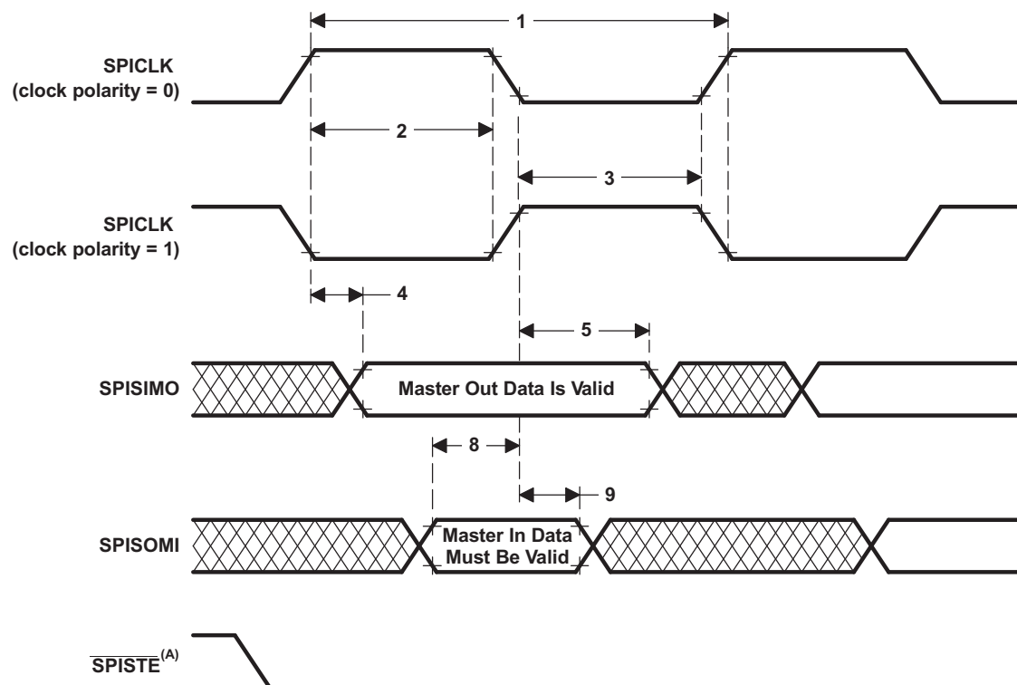
Figure 6-42. SPI Master Mode External Timing (Clock Phase = 0)
