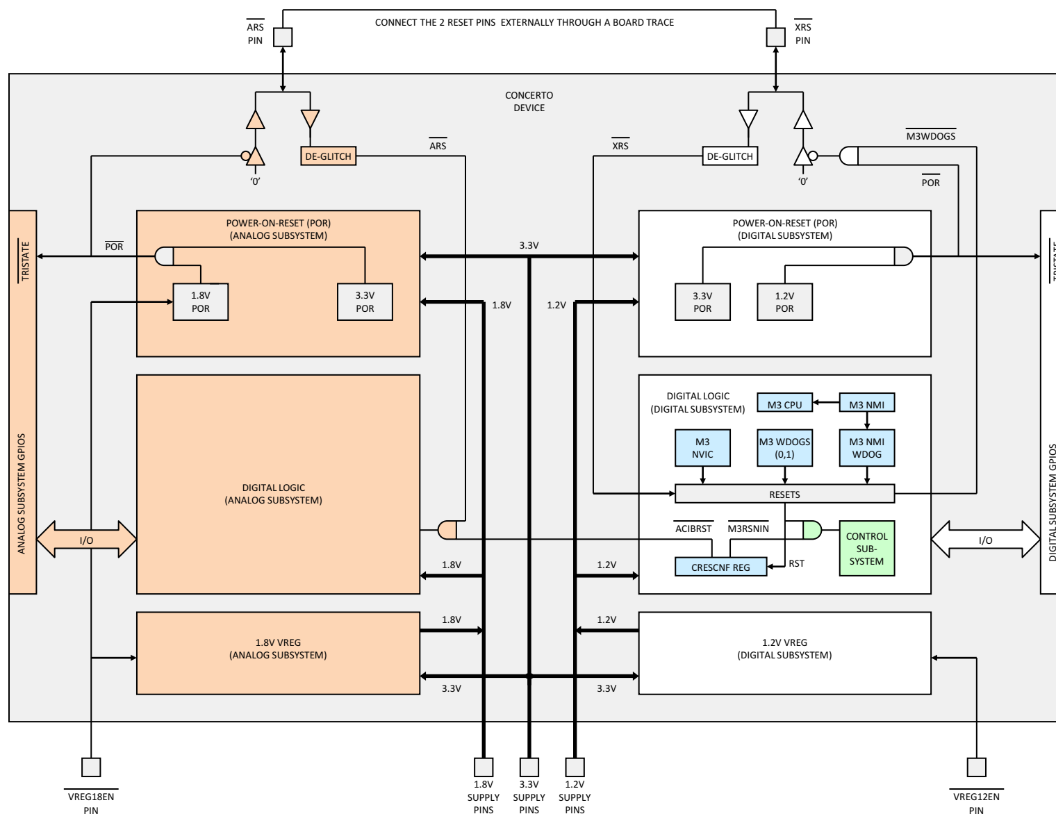
Figure 2-6. Voltage Regulation and Monitoring
