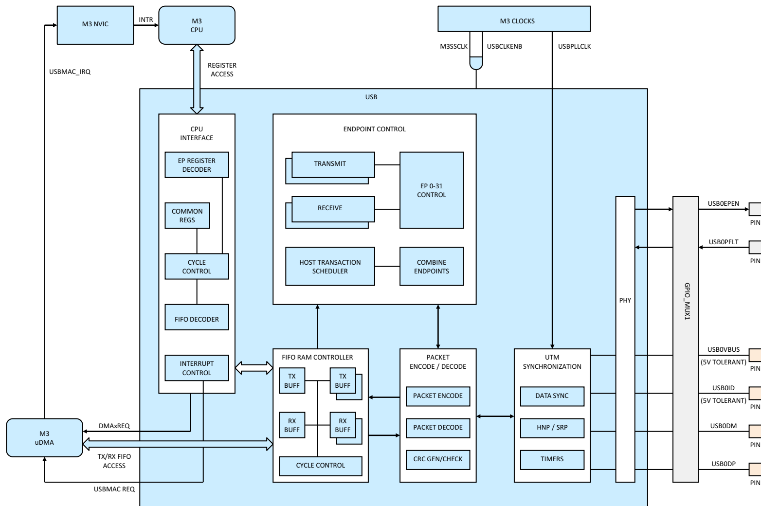
Figure 6-25. USB
