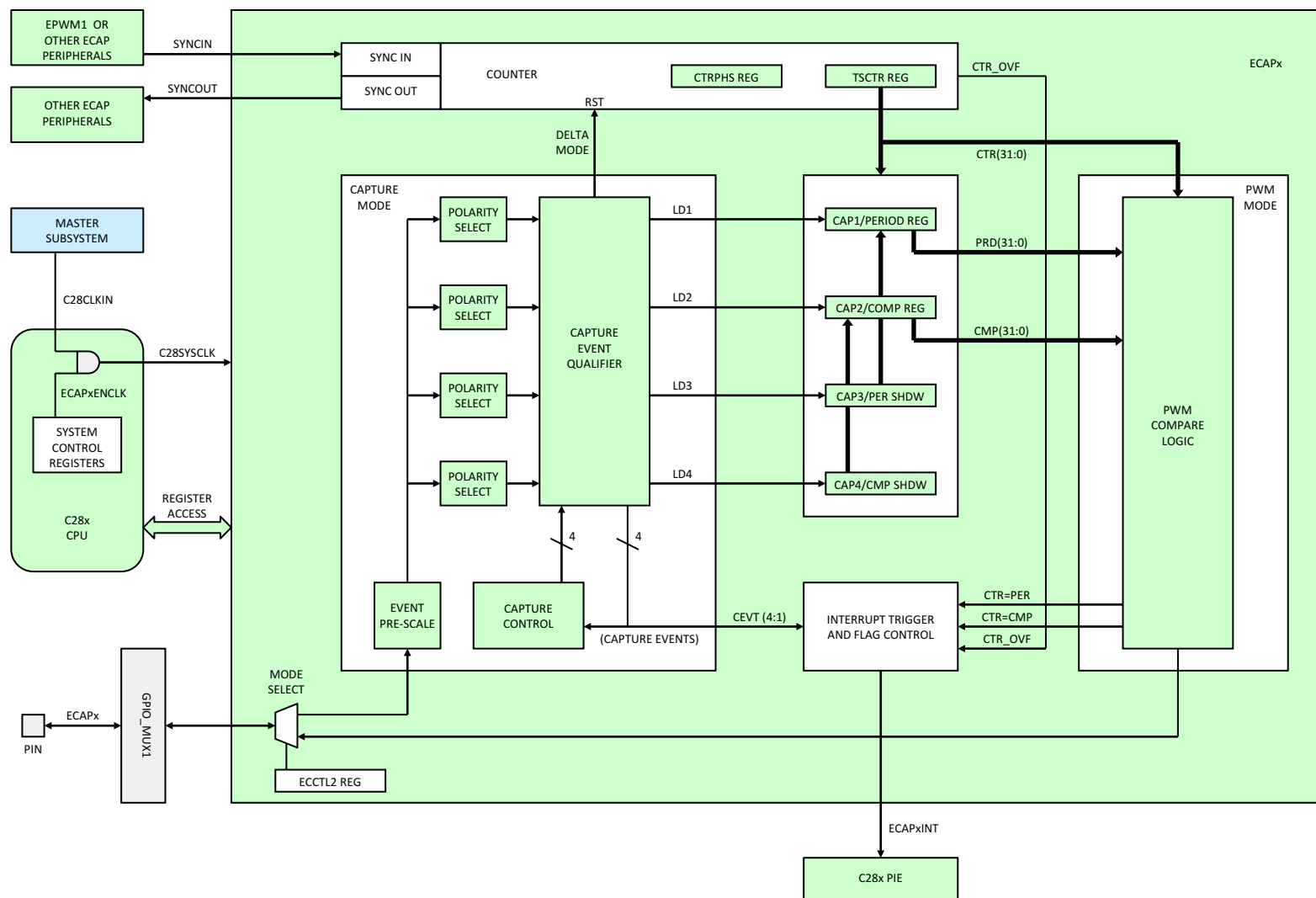
Figure 6-37. eCAP
