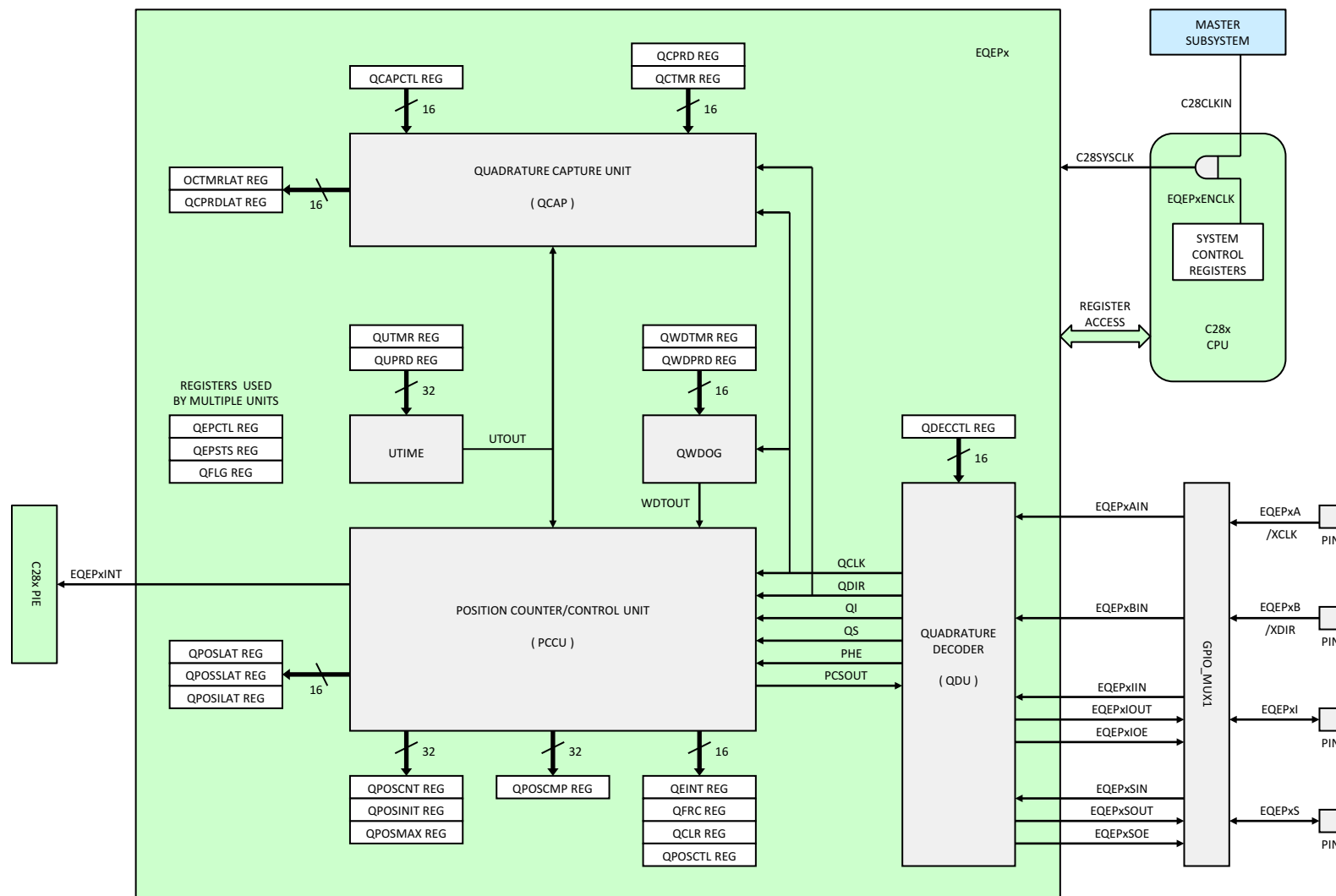
Figure 6-38. eQEP
