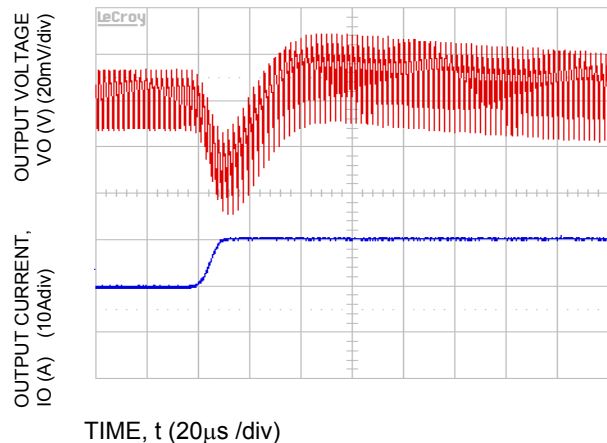
Fig-36. Transient Response to Dynamic Load Change from 50% to 100% at 12V in , C out = 2x47μF+3x330μF, C Tune =5600pF & R Tune =220ohms
