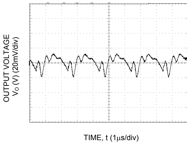
Fig-41. Typical output ripple and noise (C O =2x47μF ceramic, V IN = 12V, I o = I o,max ).
