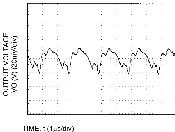
Fig-35. Typical output ripple and noise (C O =2x47μF ceramic, V IN = 12V, I O = I O,max ).
