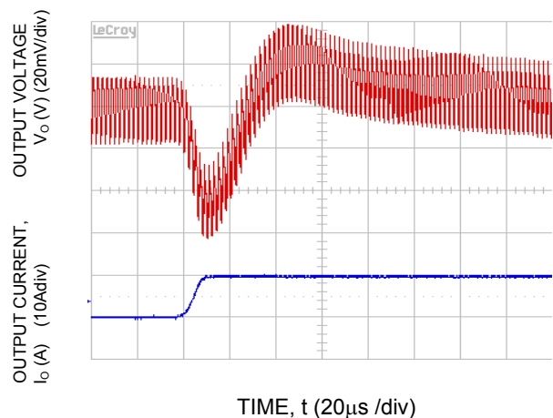
Fig-30. Transient Response to Dynamic Load Change from 50% to 100% at 12V in , C out = 2x47μF+2x330μF, C Tune =3300pF & R Tune =220ohms
