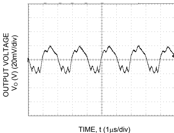
Fig-29. Typical output ripple and noise (C O =2x47μF ceramic, V IN = 12V, I o = I o,max ).
