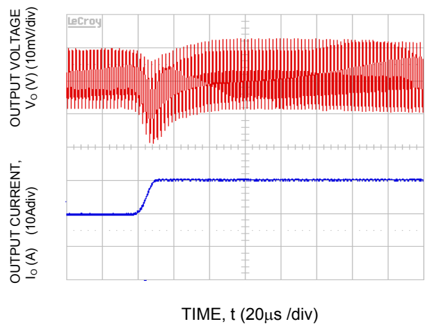
Fig-42. Transient Response to Dynamic Load Change from 50% to 100% at 12V in , C out = 1x47μF+5x330μF, C Tune =10nF & R Tune =178ohms
