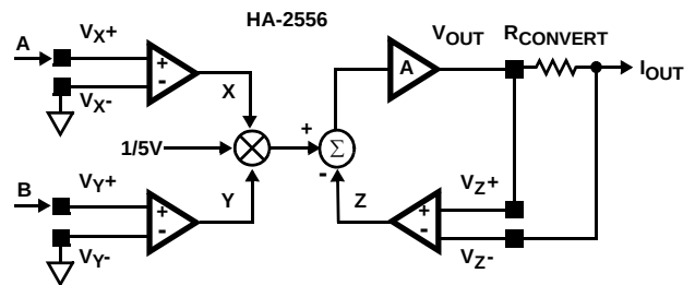
FIGURE 10. CURRENT OUTPUT
