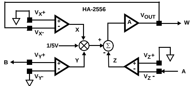
FIGURE 3. DIVIDER
