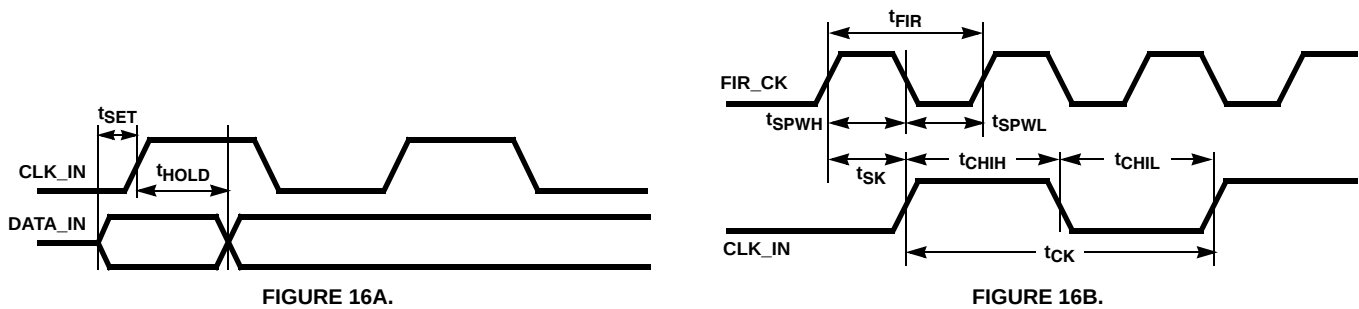
FIGURE 16. INPUT TIMING
