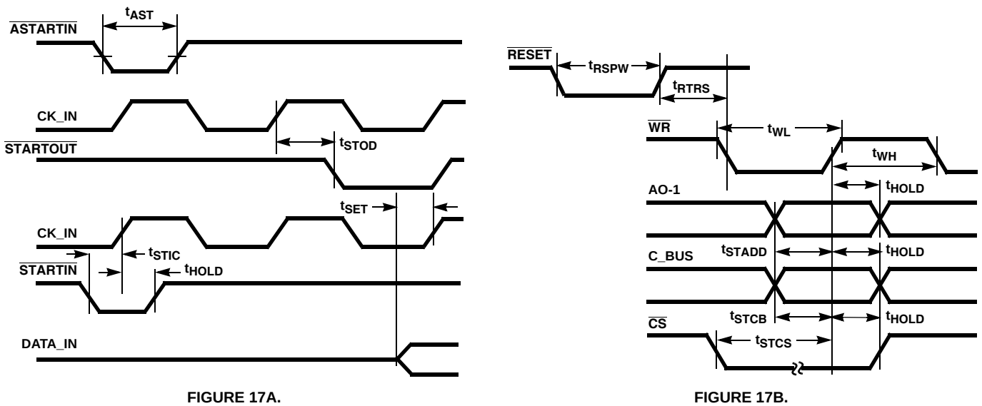
FIGURE 17. START TIMING
