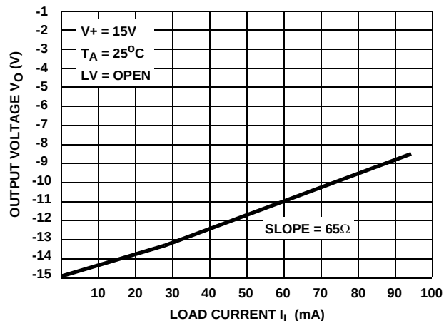
FIGURE 8. OUTPUT VOLTAGE AS A FUNCTION OF LOAD CURRENT
