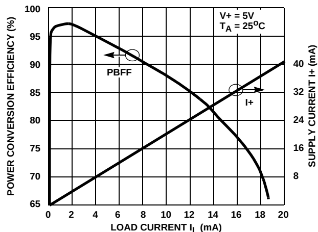
FIGURE 10. SUPPLY CURRENT AND POWER CONVERSION EFFICIENCY AS A FUNCTION OF LOAD
