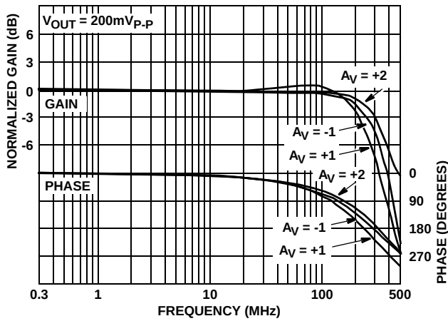
FIGURE 10. FREQUENCY RESPONSE
