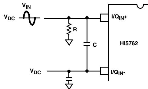
FIGURE 19. DC COUPLED SINGLE ENDED INPUT
